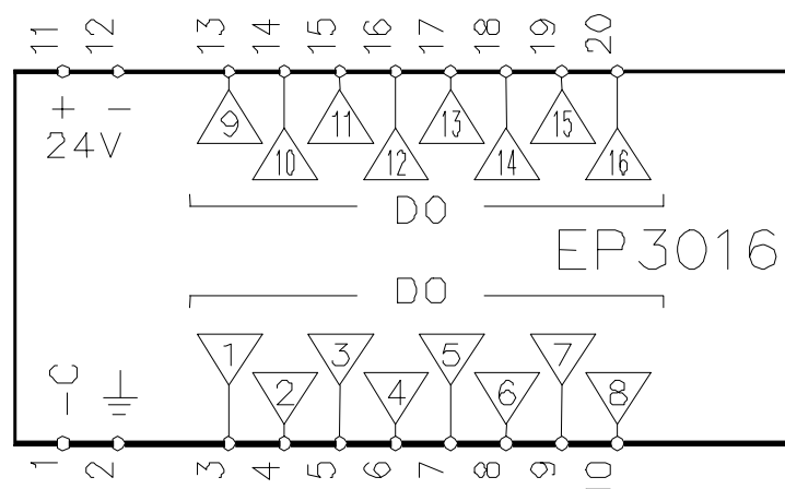
Figure 70. Connections for EP3016.
